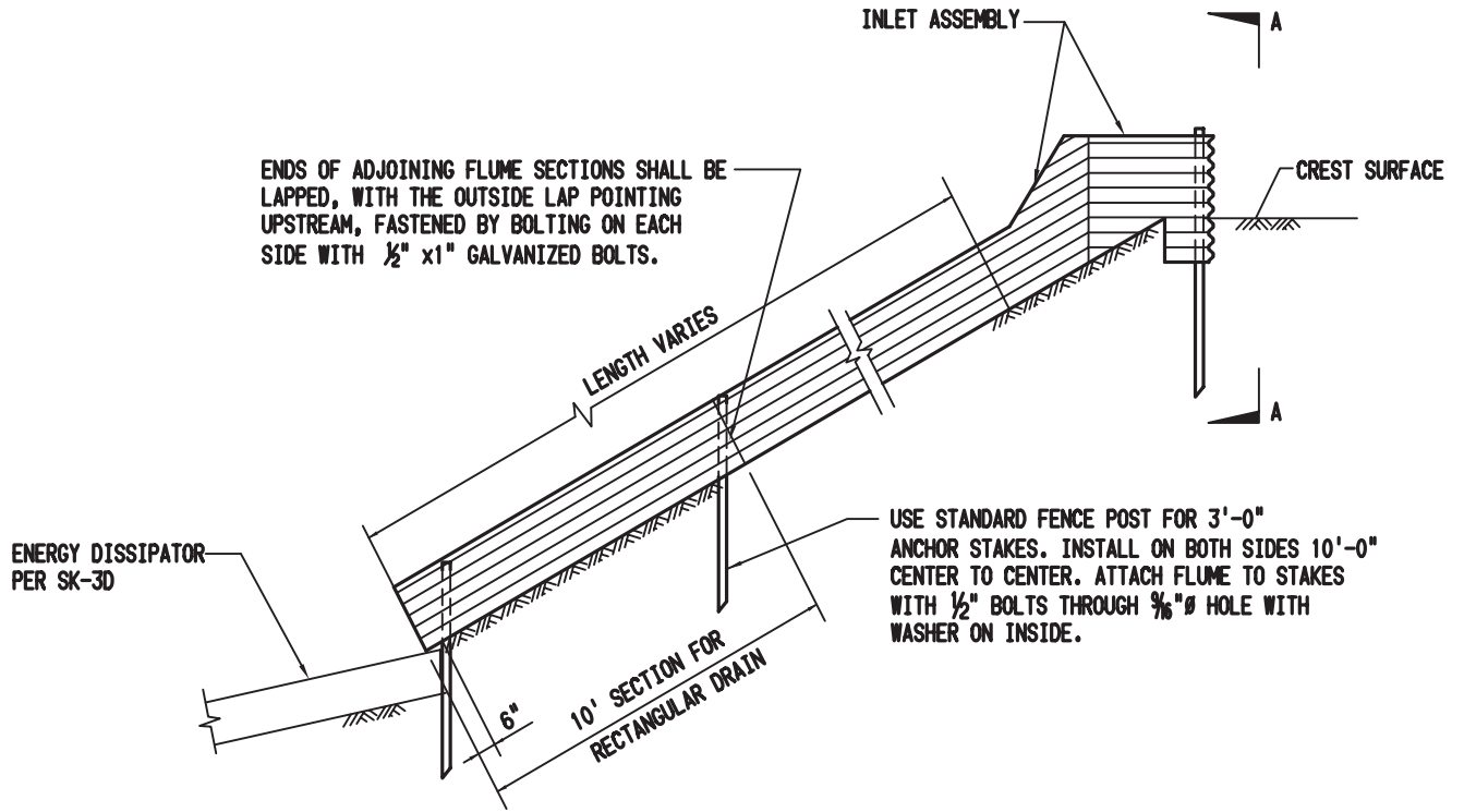
SIDE VIEW
